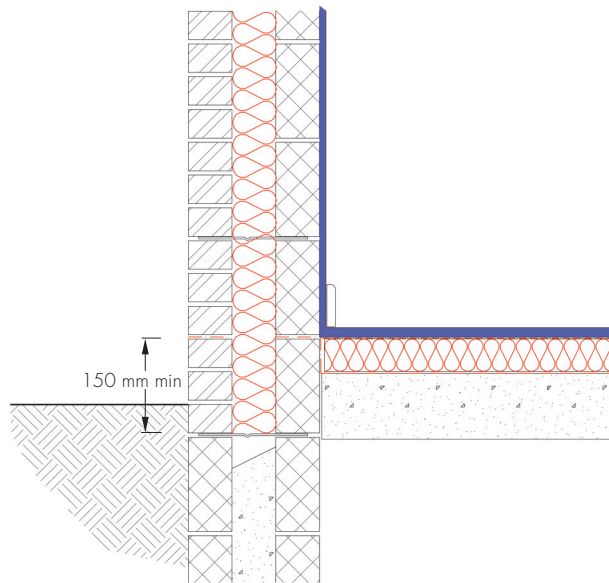
Wall-floor junction
